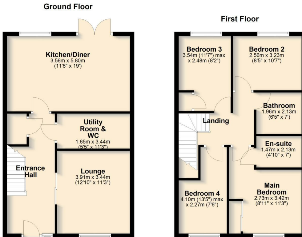
All floorplans provided are for guidance only. Please check all dimensions before making any decisions reliant upon them. Plan produced using PlanUp.
