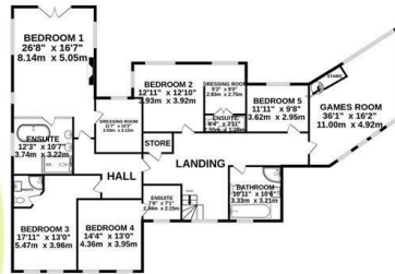
1ST FLOOR 2405 sq.ft. (223.9 sq.m.) approx.
