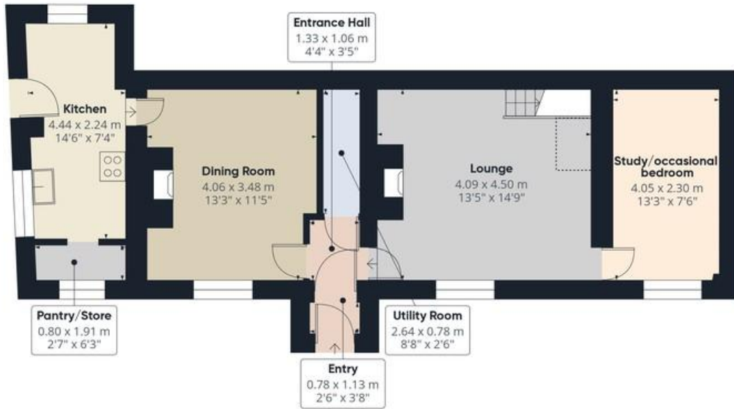
Floor 0 Building 1
