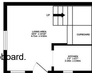
1ST FLOOR
