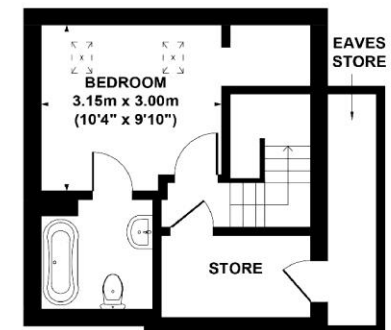
SECOND FLOOR GROSS INTERNAL FLOOR AREA 29 SQ M
