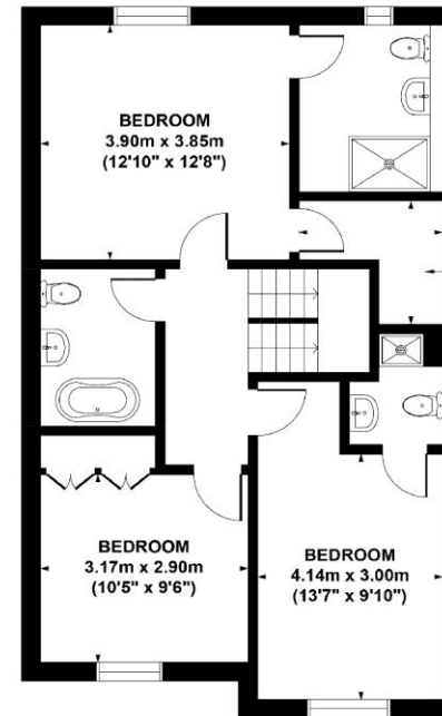
FIRST FLOOR GROSS INTERNAL FLOOR AREA 67 SQ M
