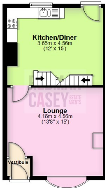
Ground Floor Approx. 36.3 sq. metres (391.0 sq. feet)
