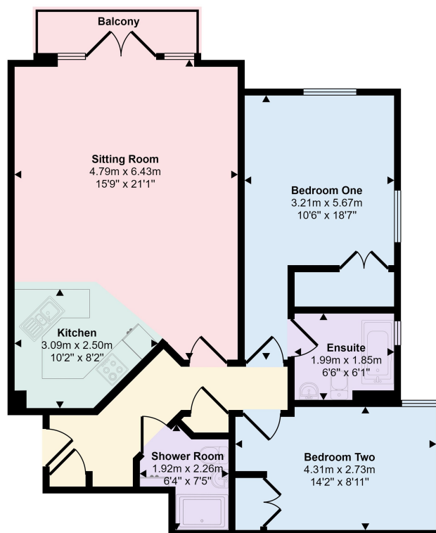
Floorplan
