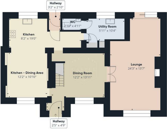
Floor 0 Building
