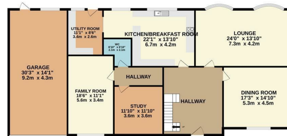
GROUND FLOOR 2060 sq.ft. (191.4 sq.m.) approx.
