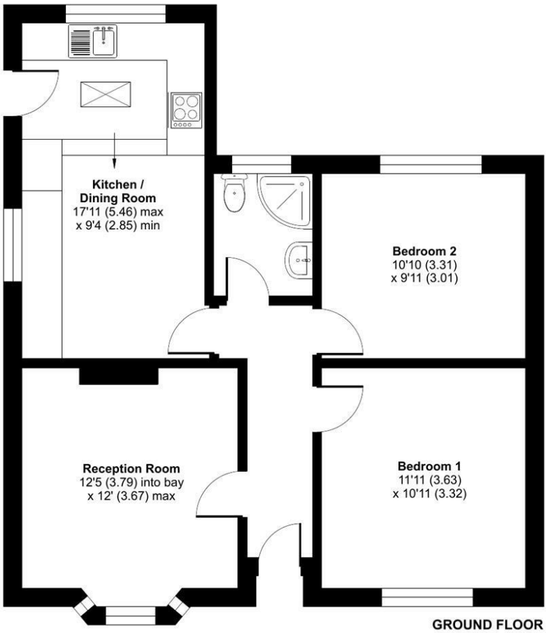
GROUND FLOOR
