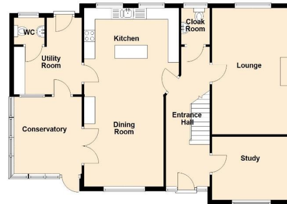
Ground Floor Approx. 151.1 sq. metres (1626.2 sq. feet)
