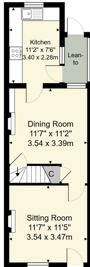
Ground Floor
