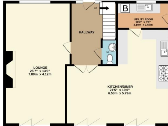
GROUND FLOOR 837 sq.ft. (77.7 sq.m.) approx.
