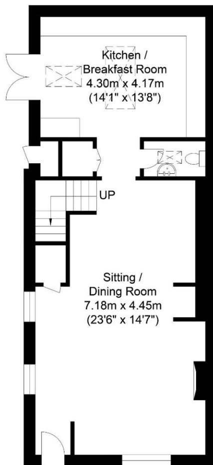
Ground Floor Approximate Floor Area 542.39 sq ft (50.39 sq m)
