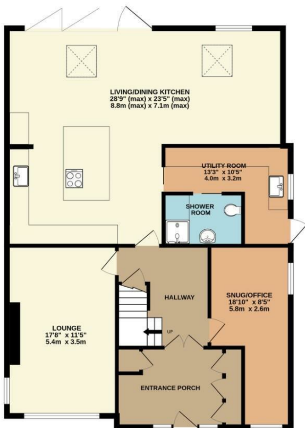
GROUND FLOOR 1190 sq.ft. (110.6 sq.m.) approx.
