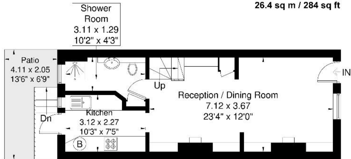
Ground Floor 38.3 sq m / 412 sq ft
