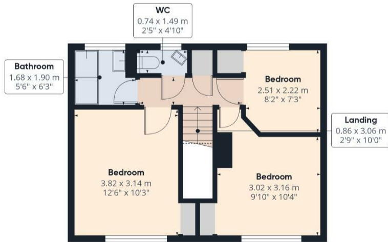
Floor 1
