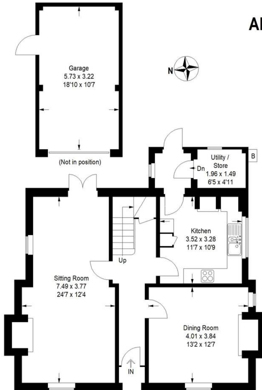
Ground Floor
