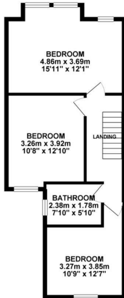
1ST FLOOR 50.19 sq. m. ( 540.24 sq. ft. )
