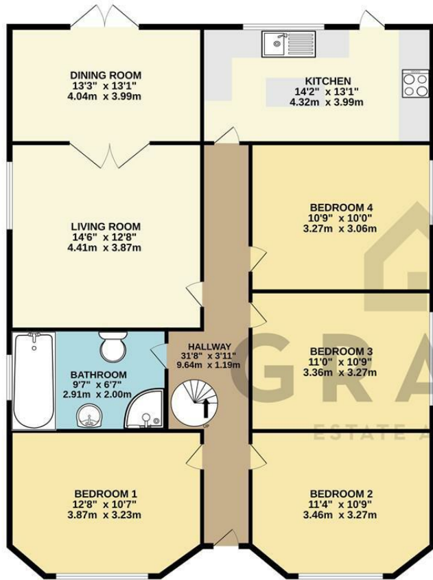
GROUND FLOOR 2241 sq.ft. (208.2 sq.m.) approx.
