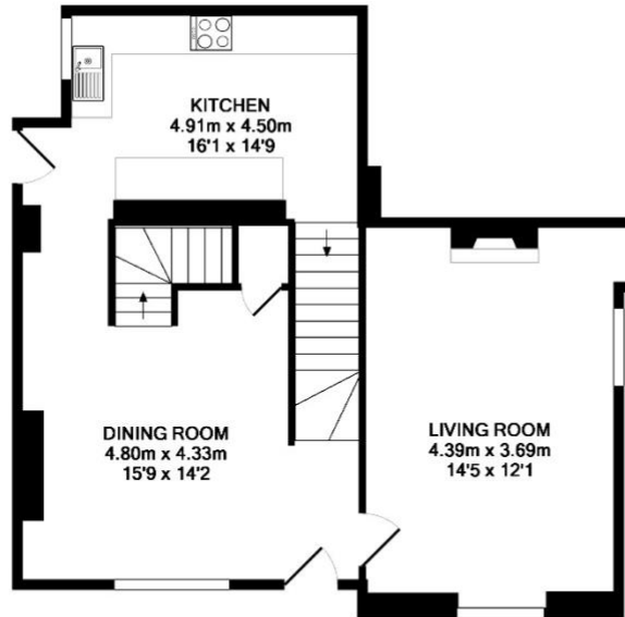
GROUND FLOOR APPROX. FLOOR AREA 57.2 SQ.M. (616 SQ.FT.)
