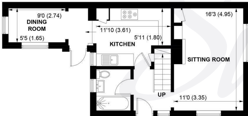
GROUND FLOOR
