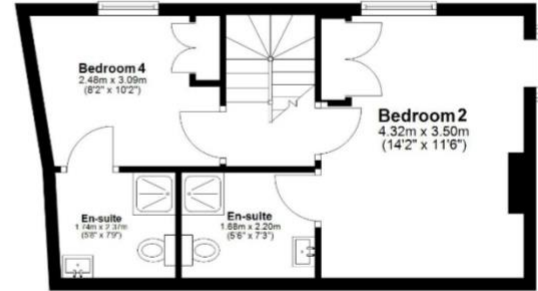
First Floor Approx. 34.4 sq. metres (370.7 sq. feet)
