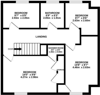
1ST FLOOR 559 sq.ft. (52.0 sq.m.) approx.
