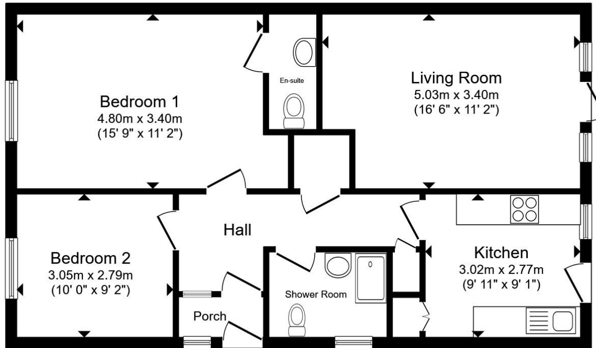
Floor Plan
