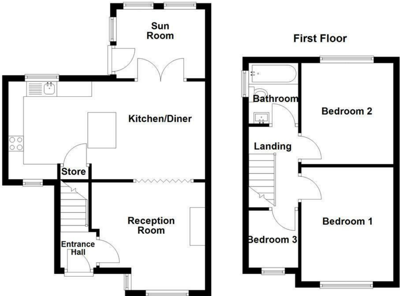
Ground Floor
