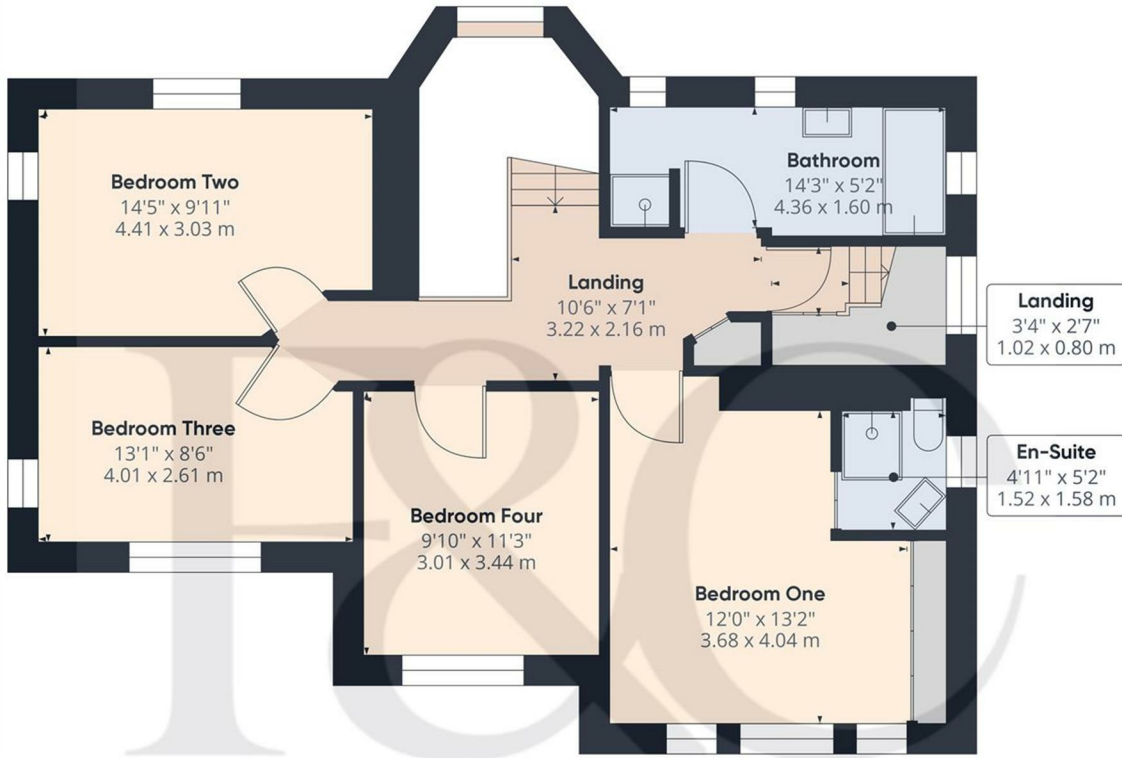
Floor 1 Building 1
