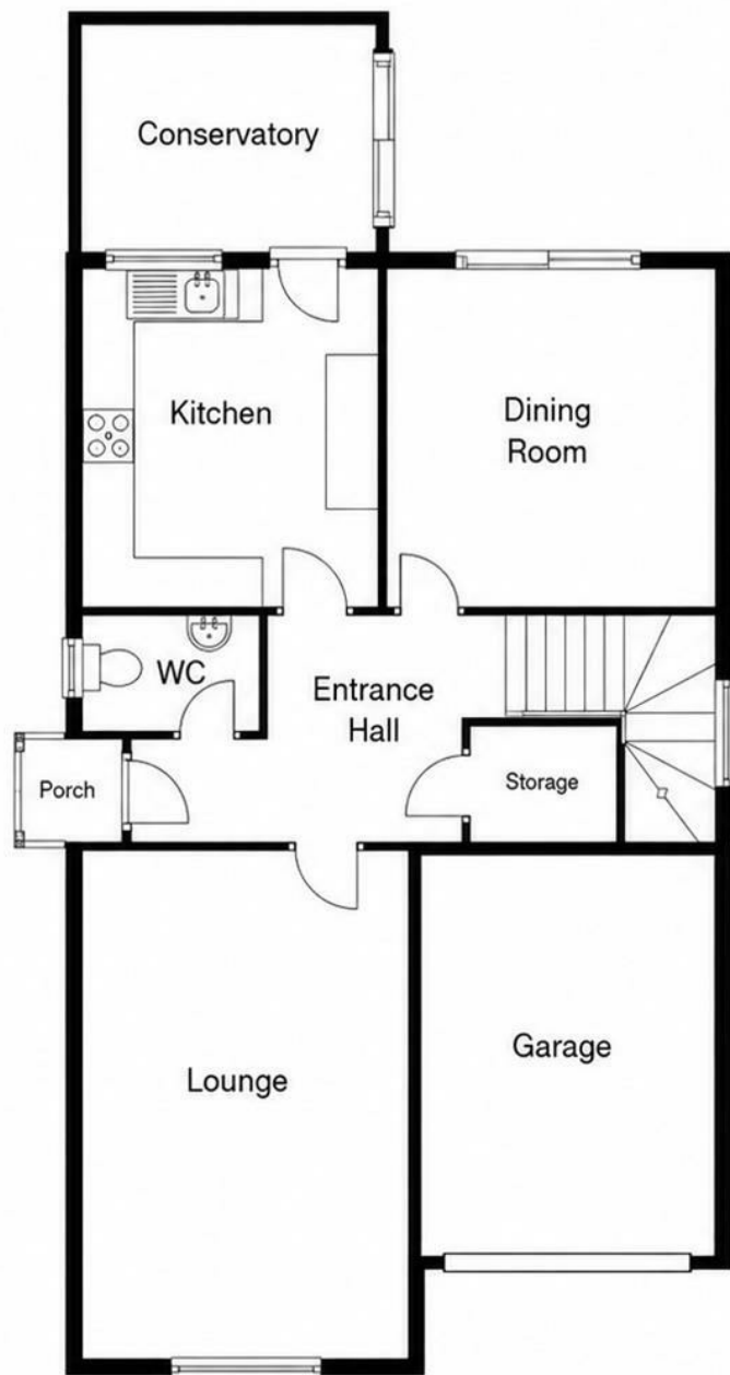
GROUND FLOOR
