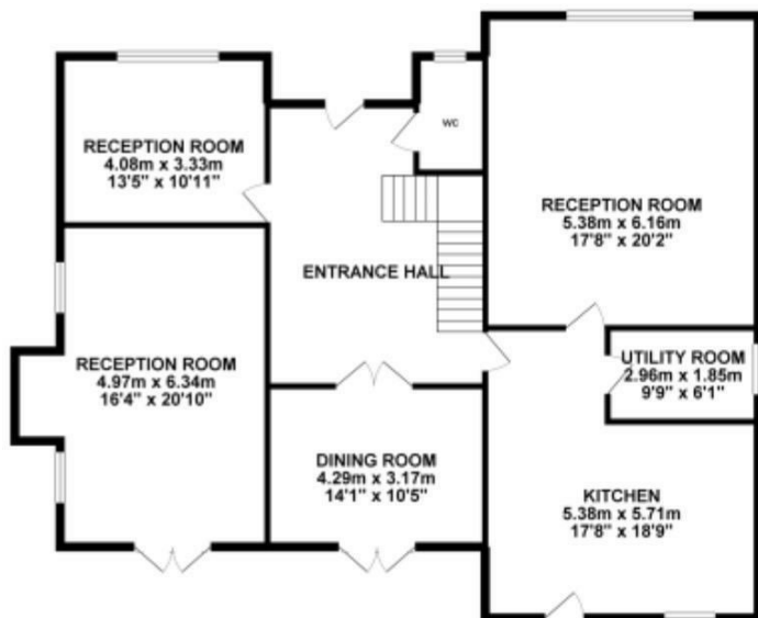
GROUND FLOOR 143.53 sq. m. ( 1544.91 sq. ft. )
