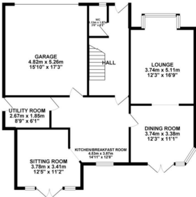
GROUND FLOOR 99.74 sq. m. ( 1073.54 sq. ft. )
