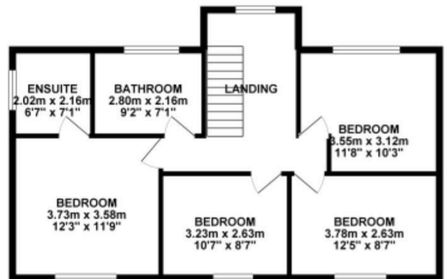
1ST FLOOR 64.13 sq. m. ( 690.32 sq. ft. )
