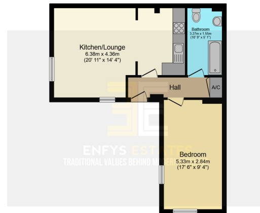
Floor Plan Floor area 51.1 sq.m. (550 sq.ft.)
