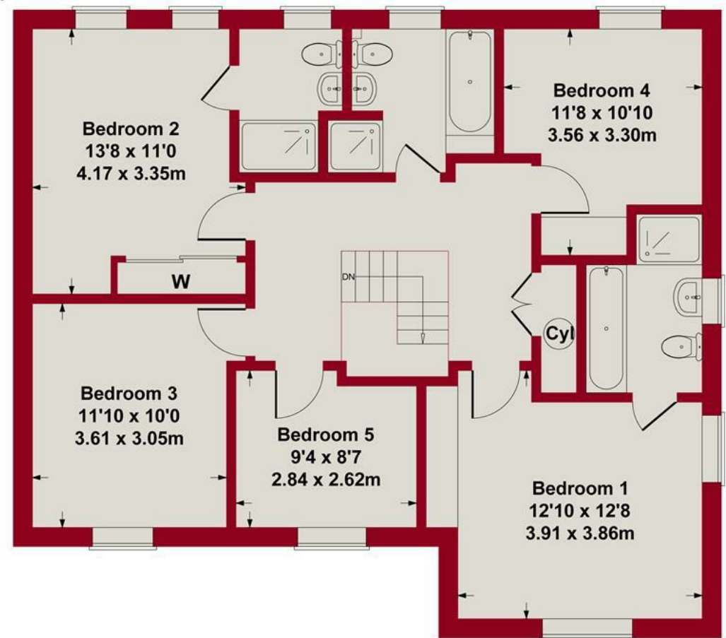
FIRST FLOOR
