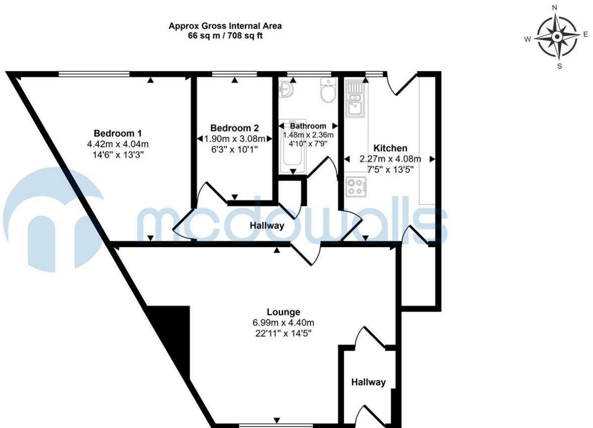
Floorplan
