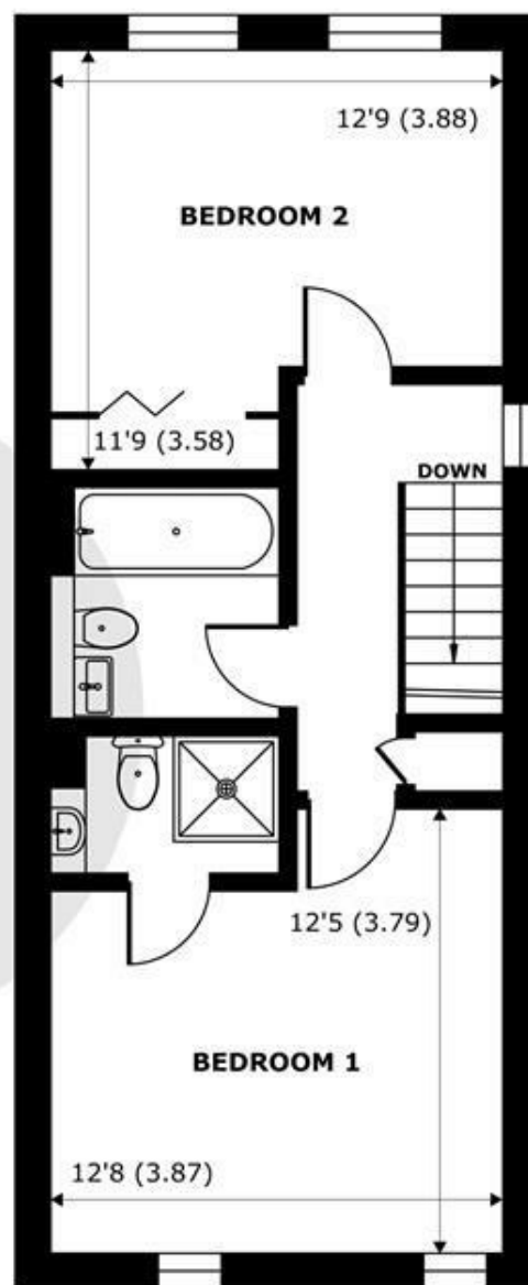
SECOND FLOOR abt 521 SQFT (48.4 SQMT)
