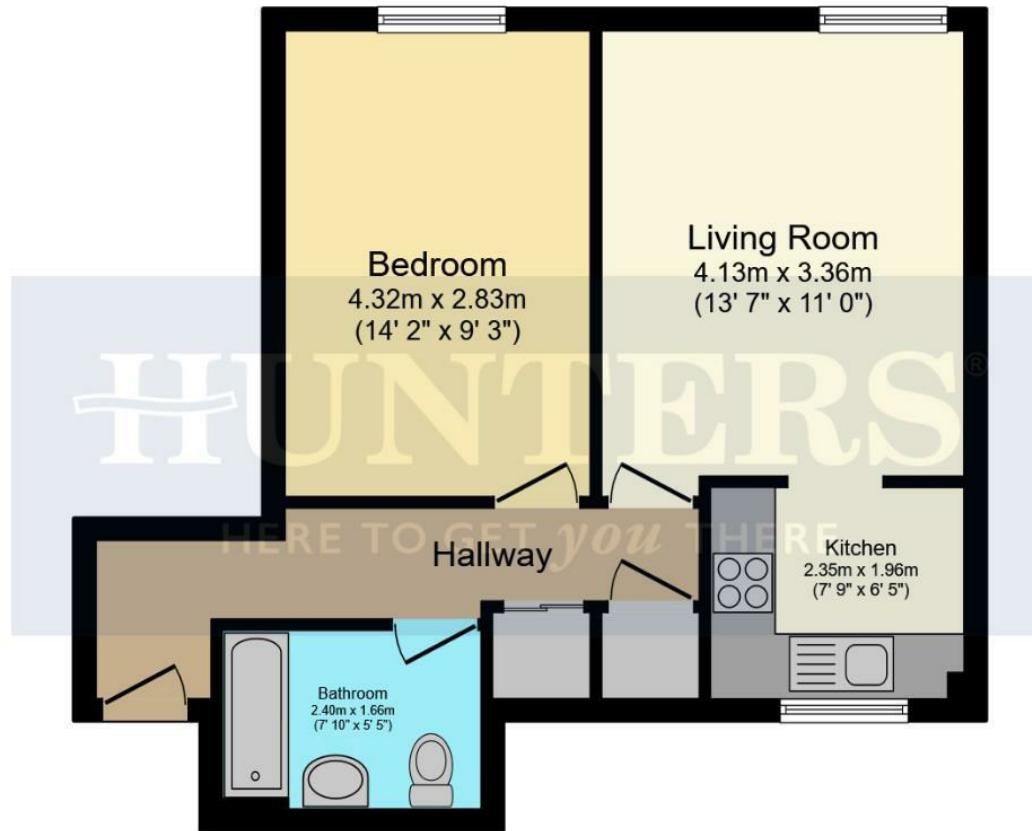
Floor Plan Floor area 42.0 sq.m. (464 sq.ft.)
