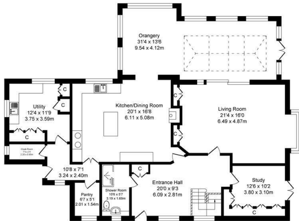
Ground Floor Approx. Floor Area 1816 Sq.Ft (168.7 Sq.M.)
