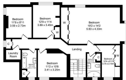
First Floor Approx. Floor Area 1138 Sq.Ft (105.7 Sq.M.)
