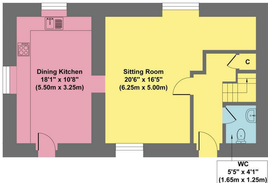
Ground Floor Approximate Floor Area 616 sq.ft (57.20 sq.m.)
