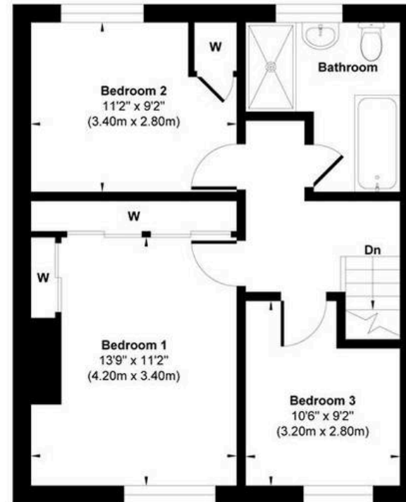
First Floor Approximate Floor Area 502 sq.ft (46.67 sq.m)
