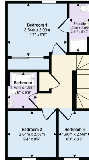
Second Floor Approx 42 sq m / 447 sq ft
