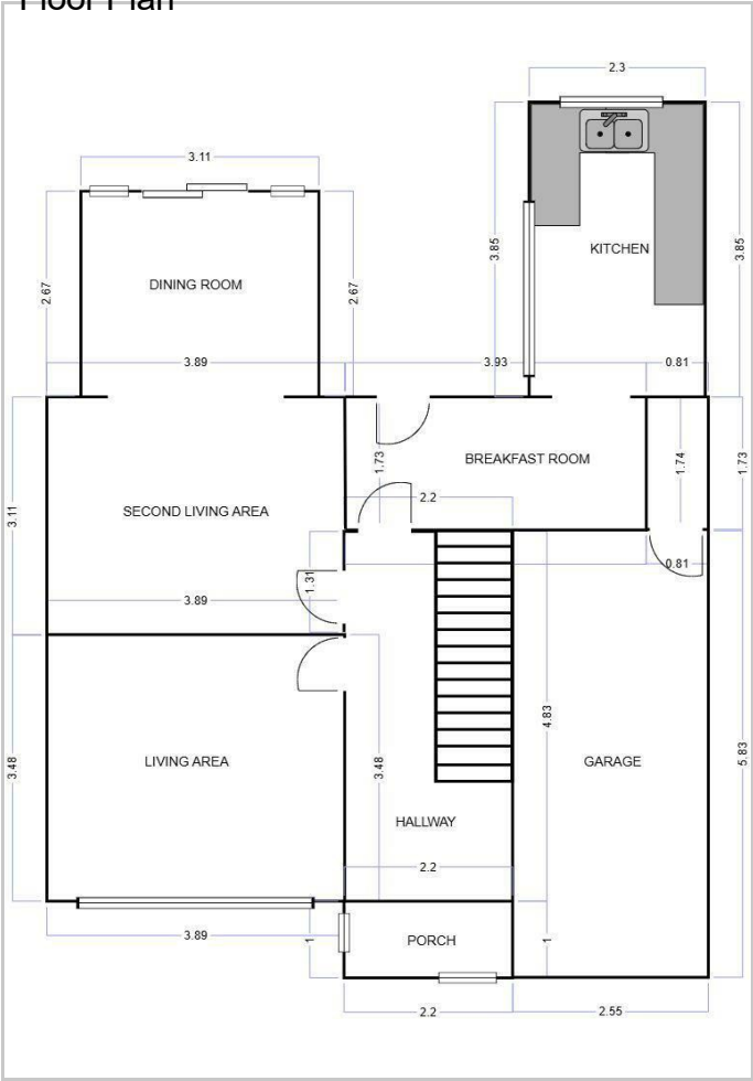
Floor Plan
