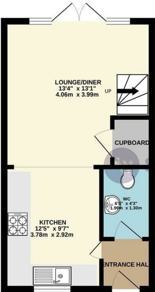
GROUND FLOOR 320 sq.ft. (29.7 sq.m.) approx.
