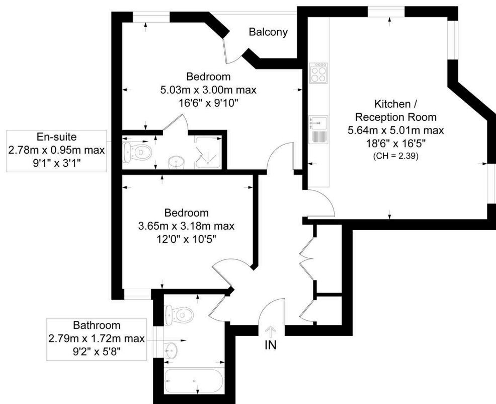
First Floor
