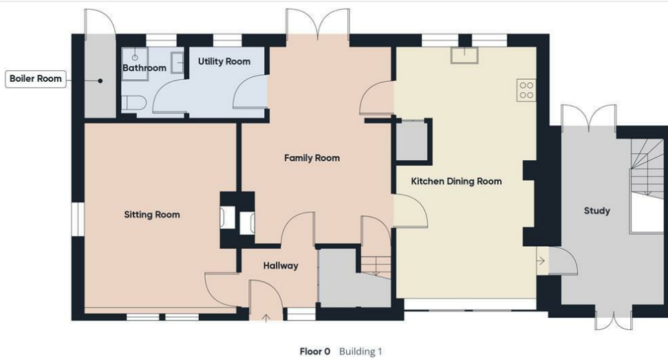
Floor 0 Building 1
