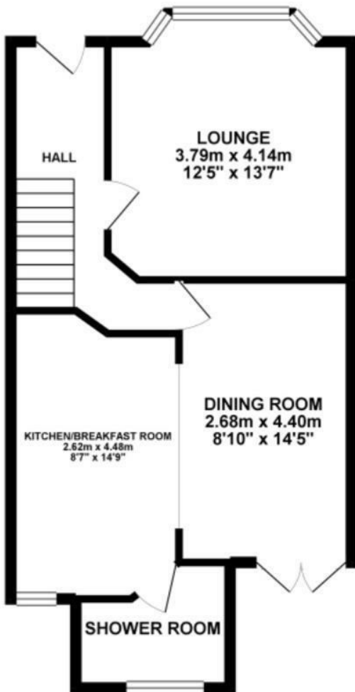
GROUND FLOOR 49.24 sq. m. ( 530.01 sq. ft. )
