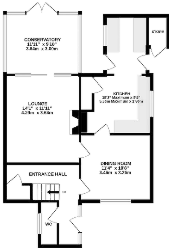
GROUND FLOOR 702 sq.ft. (65.2 sq.m.) approx.
