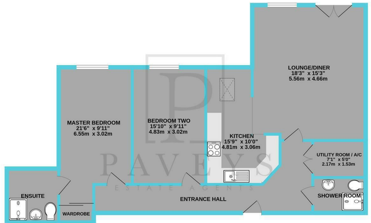
GROUND FLOOR 998 sq.ft. (92.7 sq.m.) approx.
