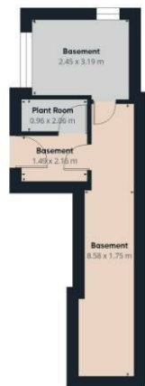
Floor -1 Building 1
