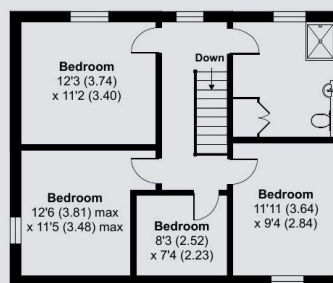
FARMHOUSE FIRST FLOOR
