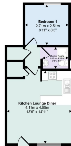
Floorplan
