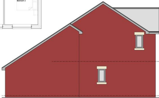
PROPOSED SIDE ELEVATION Scale 1:50 @ A1
